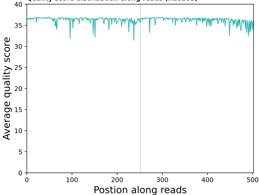
Quality score distribution along reads (R10203)
